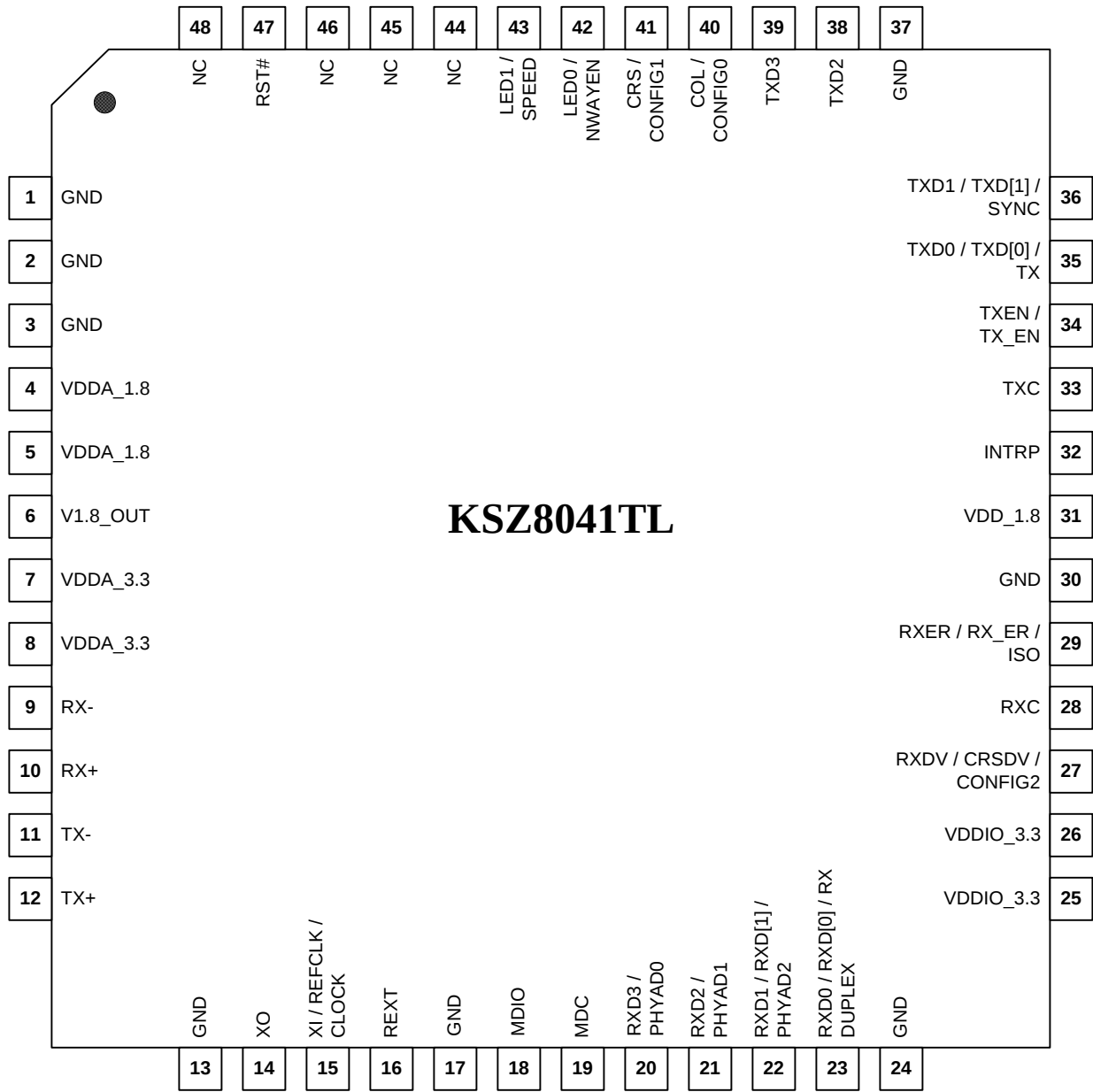
48-Pin TQFP
