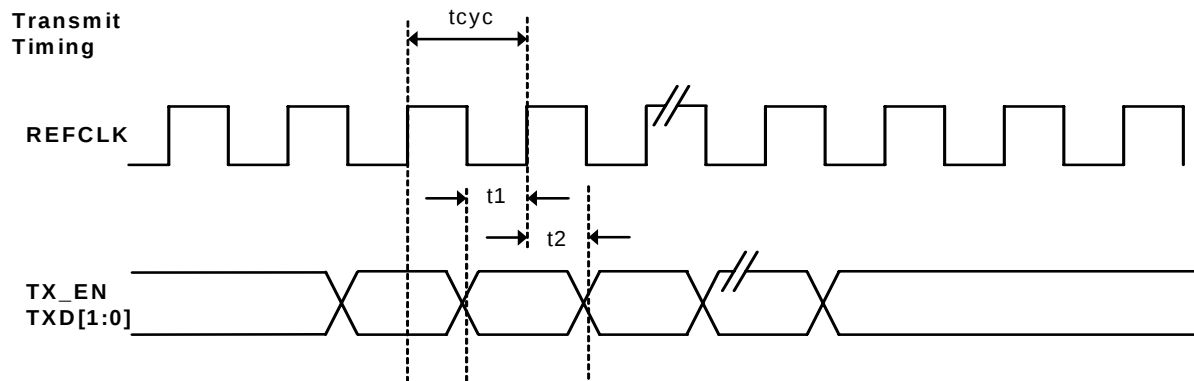
Figure 16. RMII Timing – Data Received from RMII
