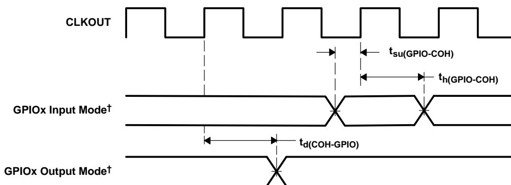
Figure 6-30. GPIOx † Timings
