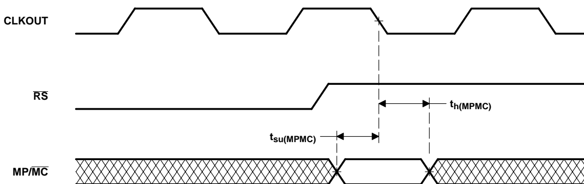
Figure 6-16. MP/MC Timing
