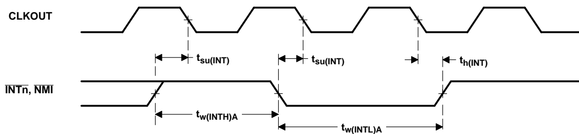
Figure 6-15. Interrupt Timing
