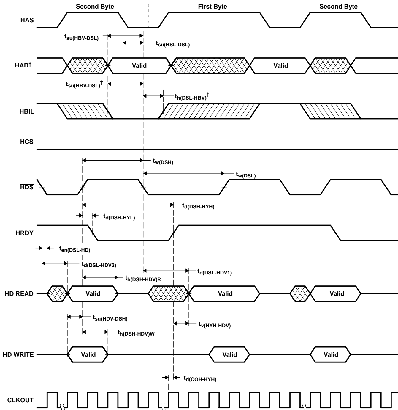
Figure 6–27. Using HDS to Control Accesses ( \overline{HCS} Always Low)
