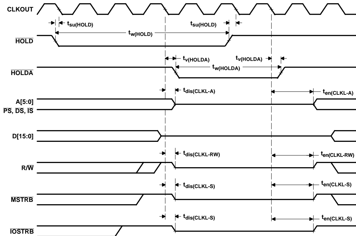
Figure 6–13. \overline{\text{HOLD}} and \overline{\text{HOLDA}} Timings (HM = 1)
