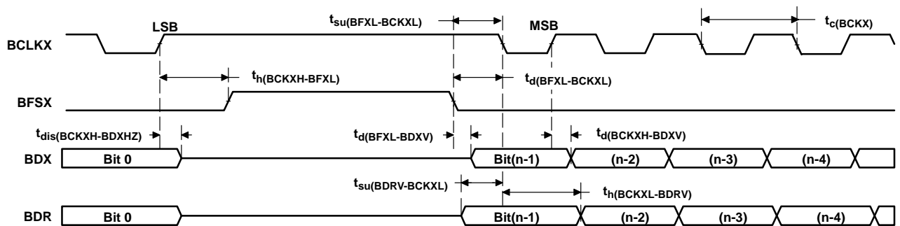
Figure 6–26. McBSP Timing as SPI Master or Slave: CLKSTP = 11b, CLKXP = 1
