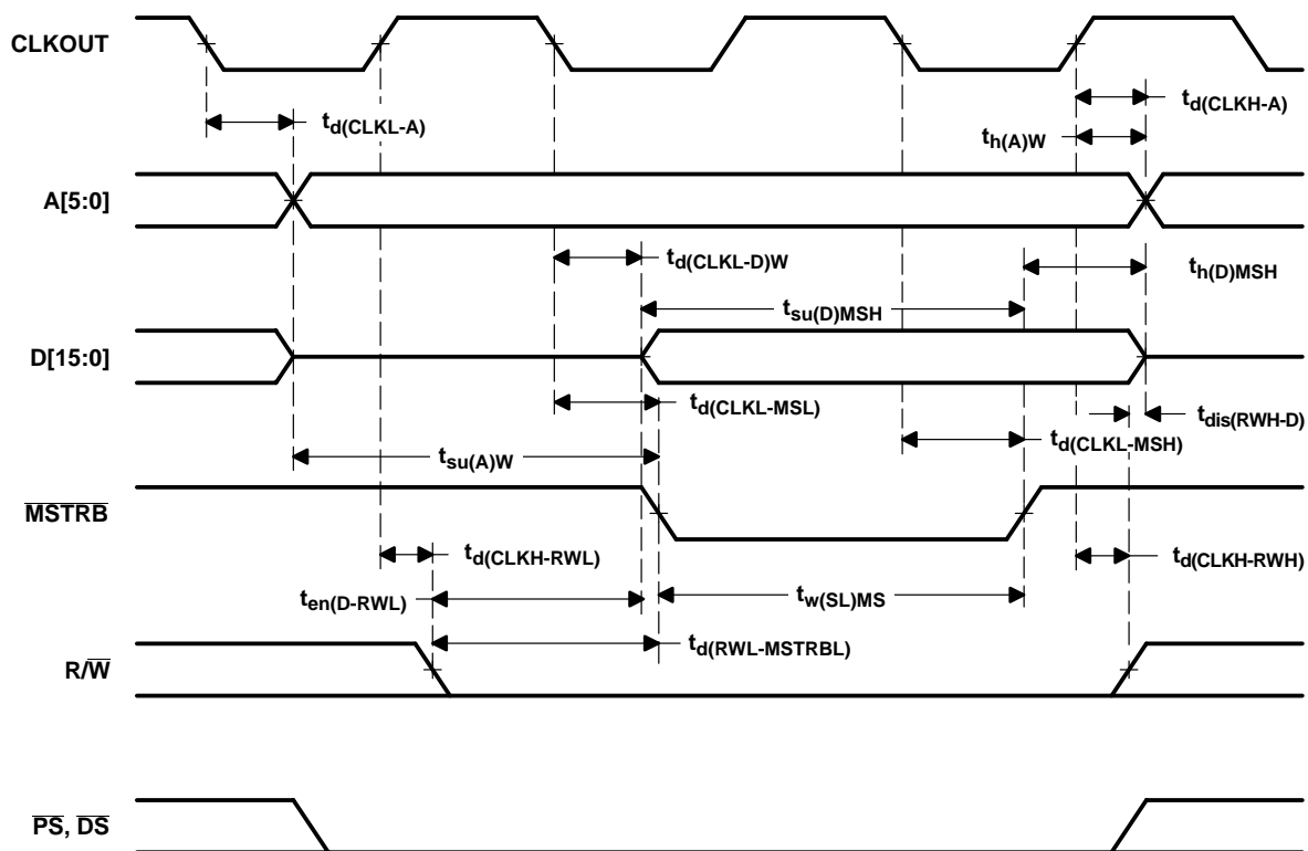
Figure 6–6. Memory Write
