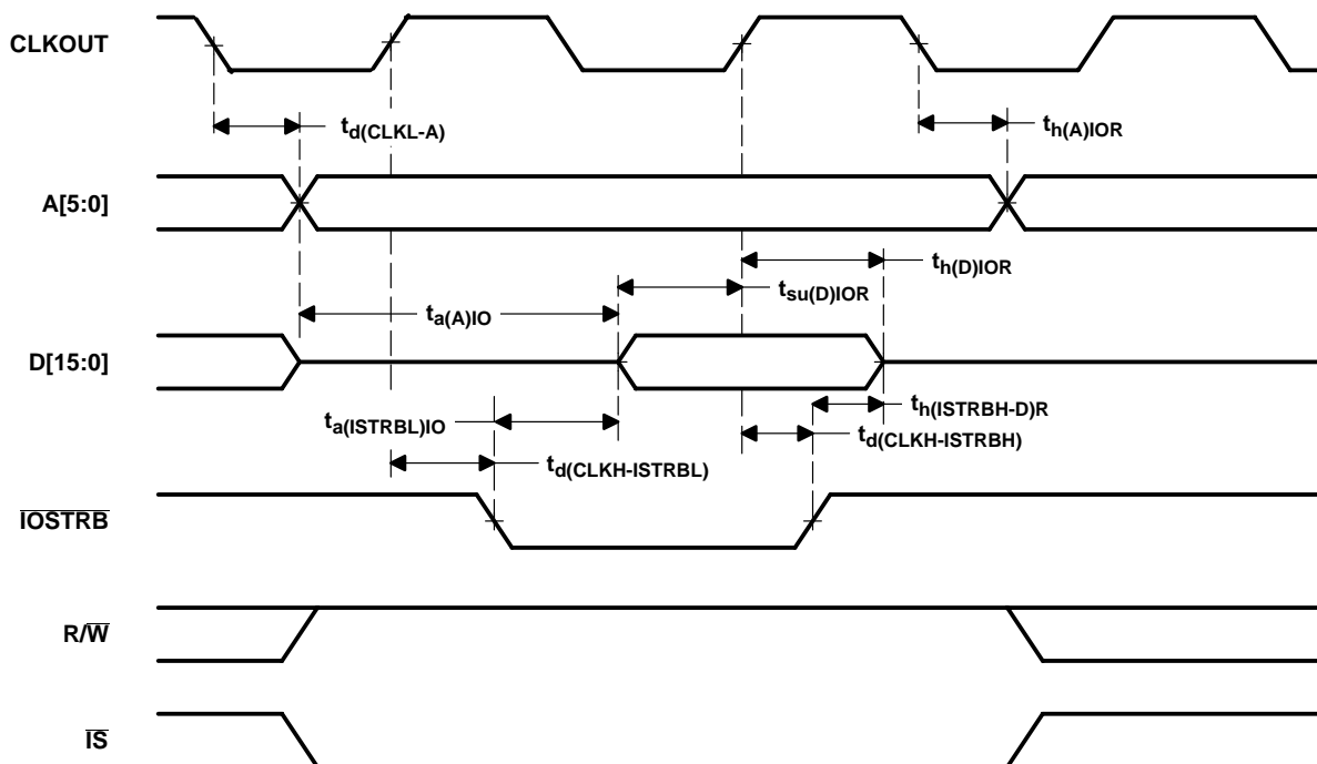
Figure 6–7. Parallel I/O Port Read
