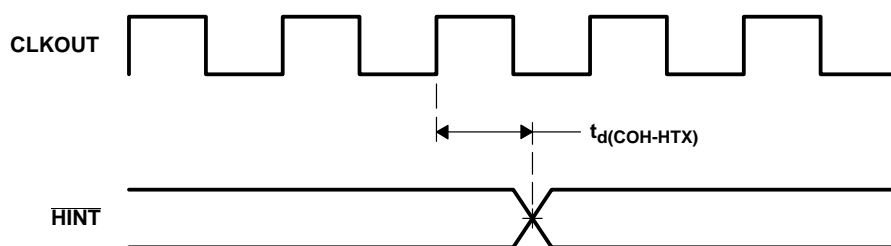
Figure 6-29. HINT Timing
