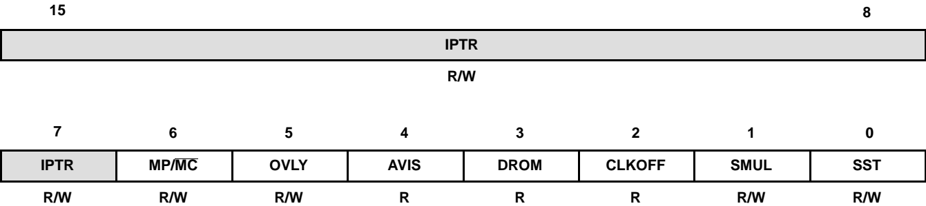
Figure 3-4. Processor Mode Status (PMST) Register
