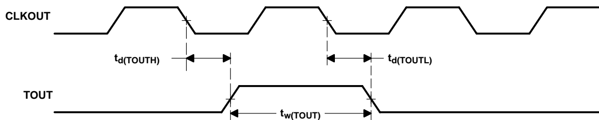
Figure 6–19. TOUT Timing
