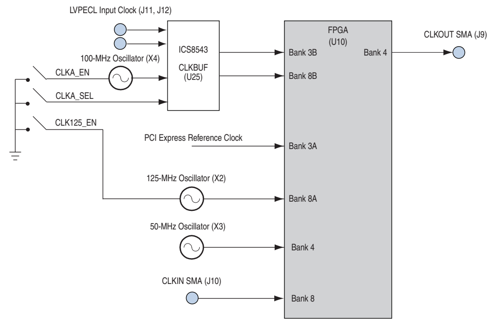
Figure 2-5. Cyclone IV GX FPGA Development Board Transceiver Clock Structure
