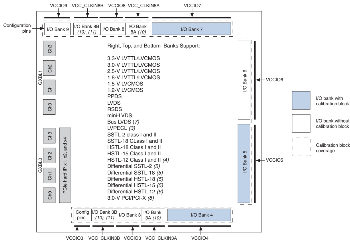
Figure 2–2. EP4CGX150DF31 Device I/O Bank Diagram (Note 1)
