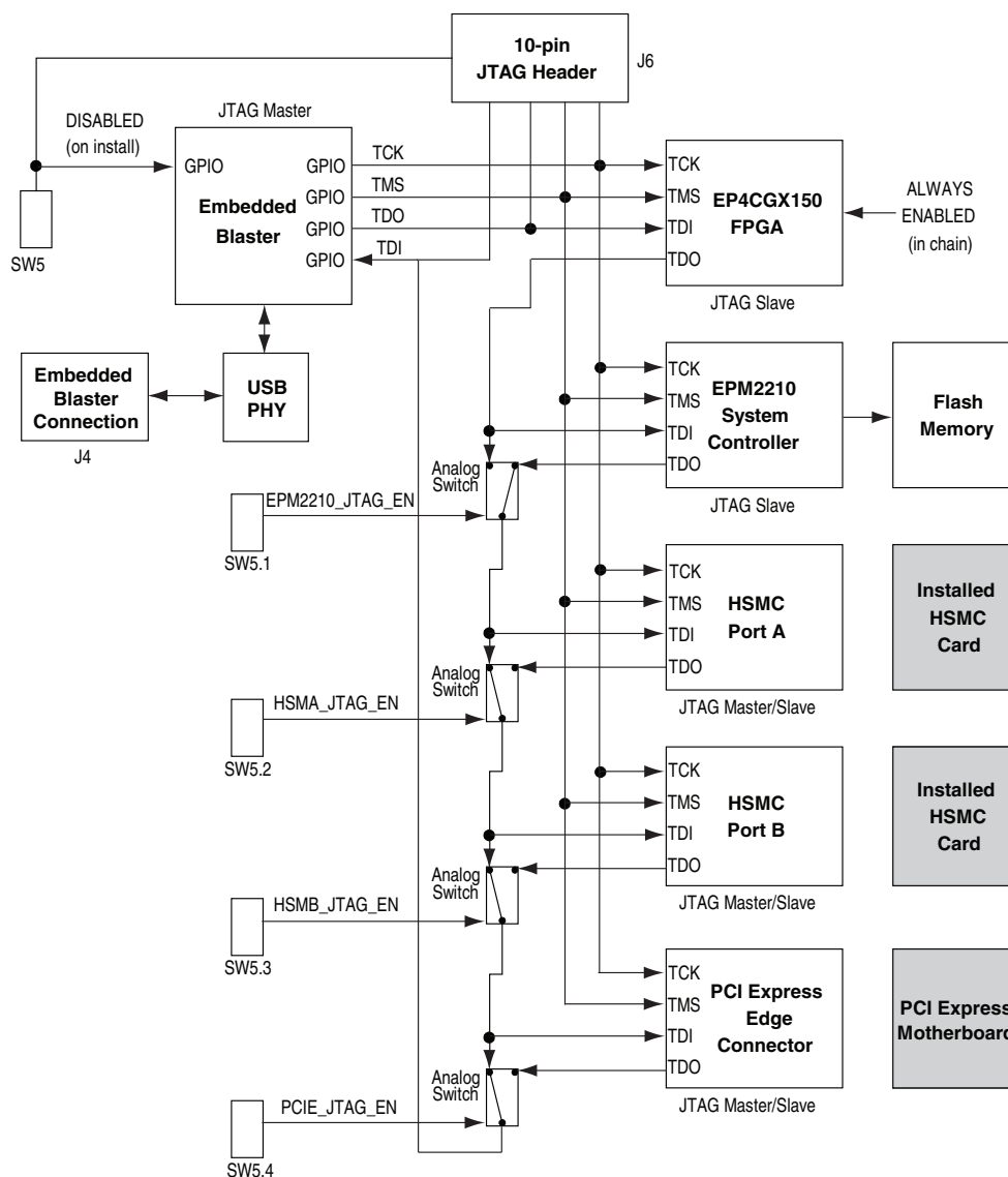
Figure 2-4. JTAG Chain
