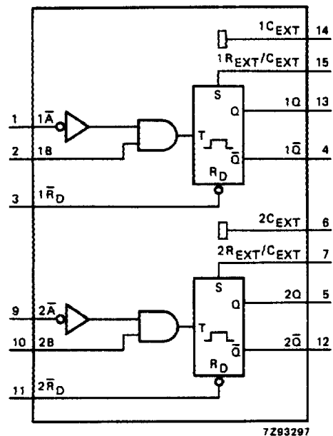
Fig.4 Functional diagram.
