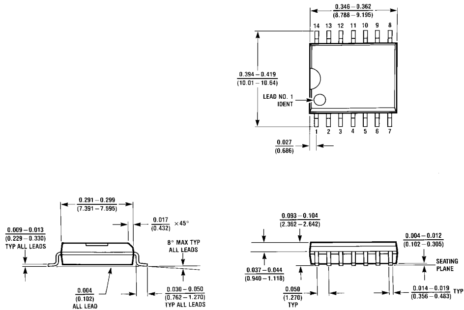
14-Lead Wide Small Outline Package (M) Order Number DM74LS243WM Package Number M14B
