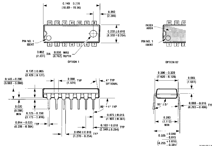
14-Lead Molded Dual-In-Line Package (N) Order Number DM74LS243N Package Number N14A
