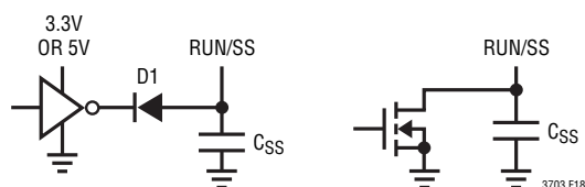
Figure 18. RUN/SS Pin Interfacing
