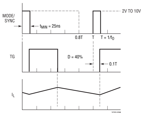
Figure 8. MODE/SYNC Clock Input and Switching Waveforms for Synchronous Operation
