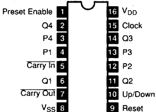
NTE4516B 16-Lead DIP, See Diag. 249 Presetable Up/Down Binary Counter
