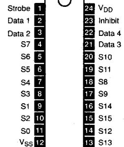
NTE4514B, NTE4515B 24-Lead DIP, See Diag. 252 4-Bit Latch/4-to-16 Line Decoder
