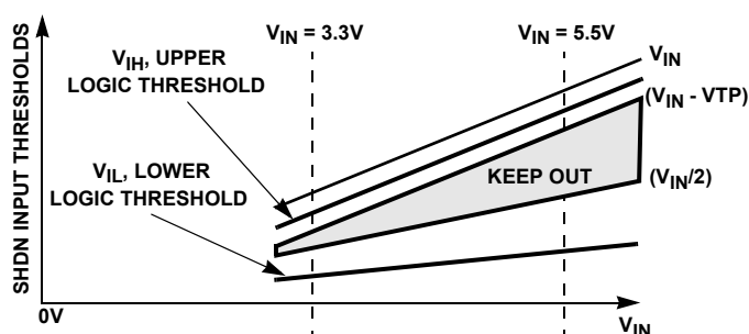
FIGURE 32. SHDN INPUT THRESHOLD vs INPUT SUPPLY VOLTAGE
