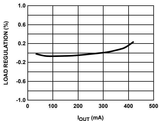
FIGURE 8. LOAD REGULATION - 3.3V V_{IN} TO 9V V_{OUT} @ 600kHz
