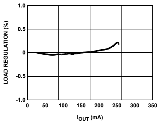
FIGURE 4. LOAD REGULATION - 3.3V V_{IN} TO 12V V_{OUT} @ 620kHz
