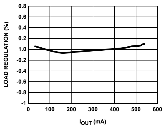
FIGURE 12. LOAD REGULATION - 5V V_{IN} TO 12V V_{OUT} @ 600kHz
