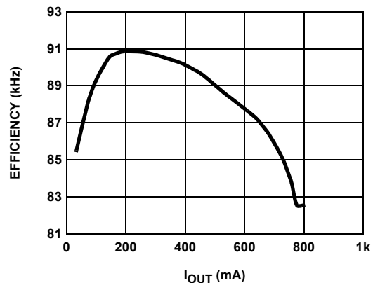
FIGURE 22. EFFICIENCY - 5V V_{IN} TO 9V V_{OUT} @ 600kHz
