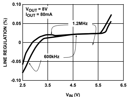
FIGURE 16. LINE REGULATION
