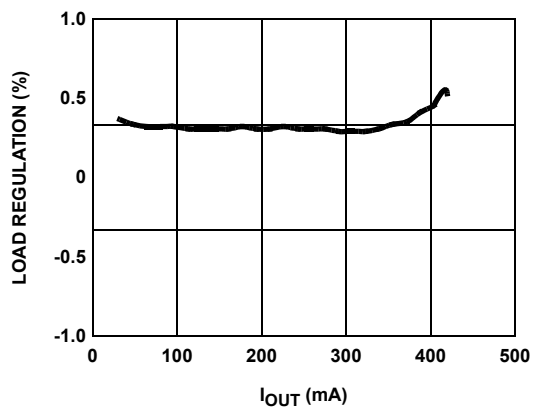
FIGURE 6. LOAD REGULATION - 3.3V V_{IN} TO 9V V_{OUT} @ 1.2MHz
