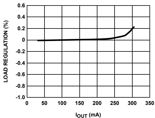
FIGURE 2. LOAD REGULATION - 3.3V V_{IN} TO 12V V_{OUT} @ 1.3MHz
