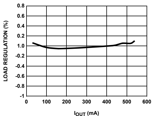
FIGURE 10. LOAD REGULATION - 5V V_{IN} TO 12V V_{OUT} @ 1.2MHz
