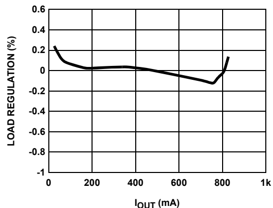
FIGURE 14. LOAD REGULATION - 5V V_{IN} TO 9V V_{OUT} @ 1.2MHz
