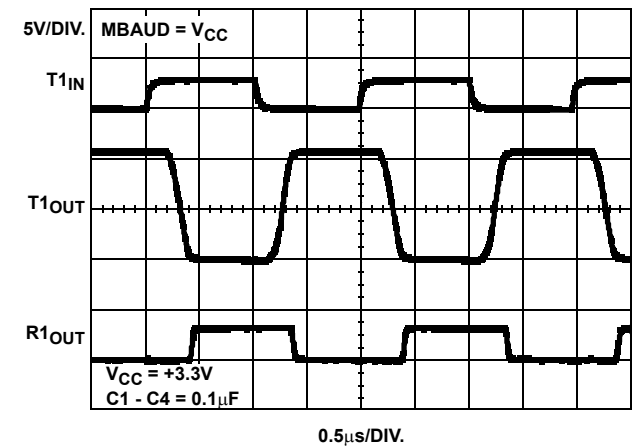
FIGURE 7. LOOPBACK TEST AT 1Mbps (CL = 250pF)
