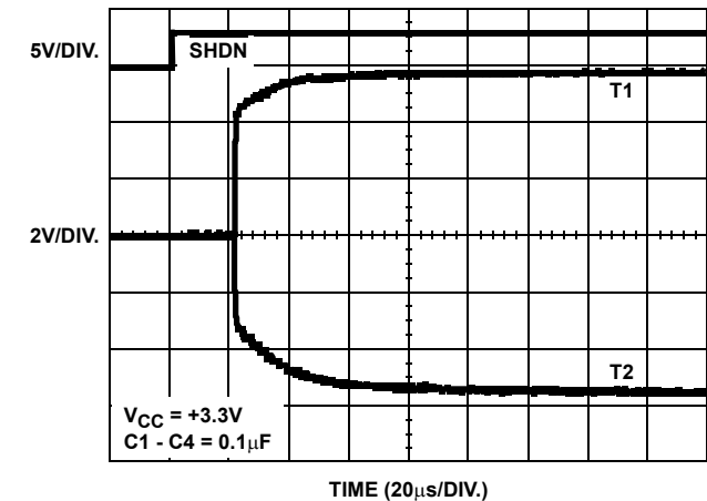
FIGURE 4. TRANSMITTER OUTPUTS WHEN EXITING POWERDOWN
