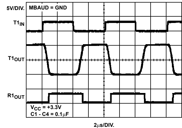
FIGURE 6. LOOPBACK TEST AT 250kbps (CL = 1000pF)
