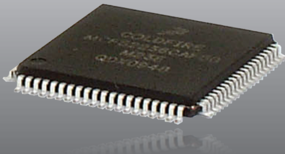
CHIP Version with 80-pin LQFP
