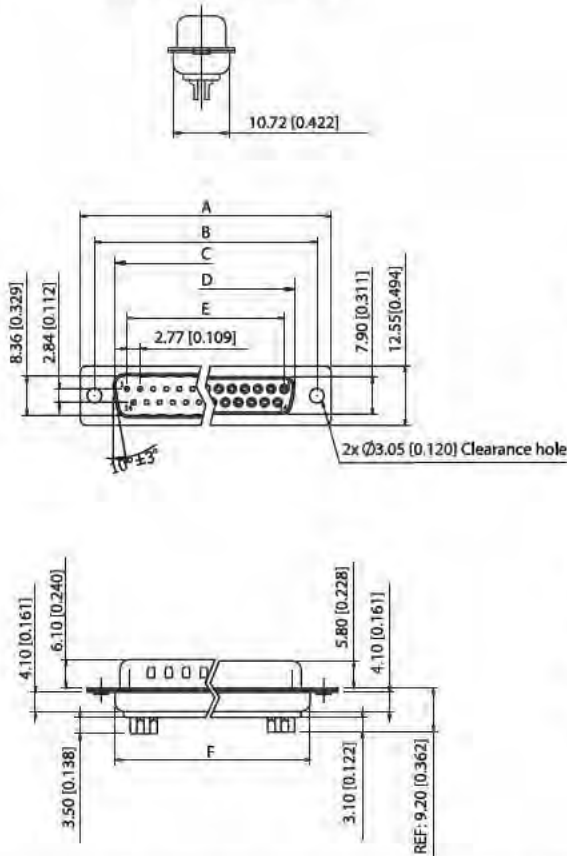
9,15,25,37 Positions
