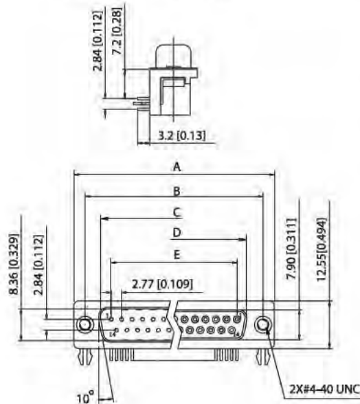
7.2mm[0.28"] Footprint
