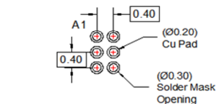
RECOMMENDED LAND PATTERN (NSMD PAD TYPE)
