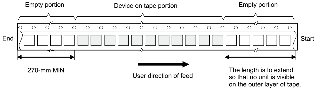
Figure 7-2. Carrier Tape and Pockets
