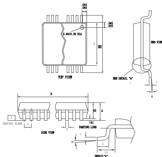
56 PIN SSOP-300mil
