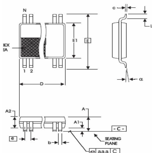
56 PIN TSSOP-240mil
