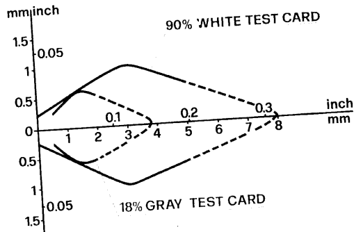
OF-26/OF-28 Proximity scanner
