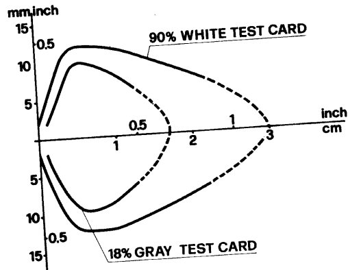
OF-18/OF-22/OF-24 Proximity scanner
