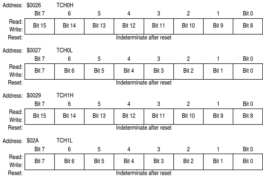
Figure 14-9. TIM Channel Registers (TCH0H/L:TCH1H/L)
