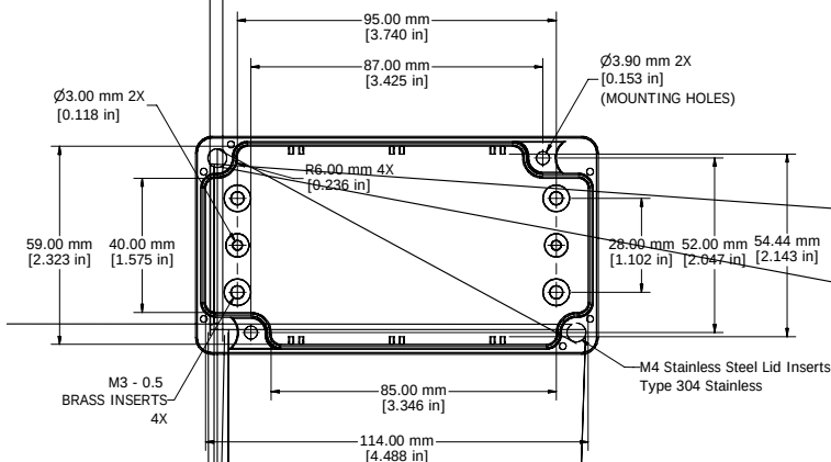
BOX - INSIDE
