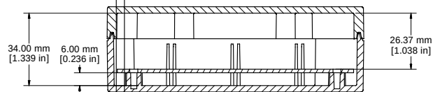
SECTION B-B
