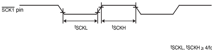
Figure 14-3 External Clock
