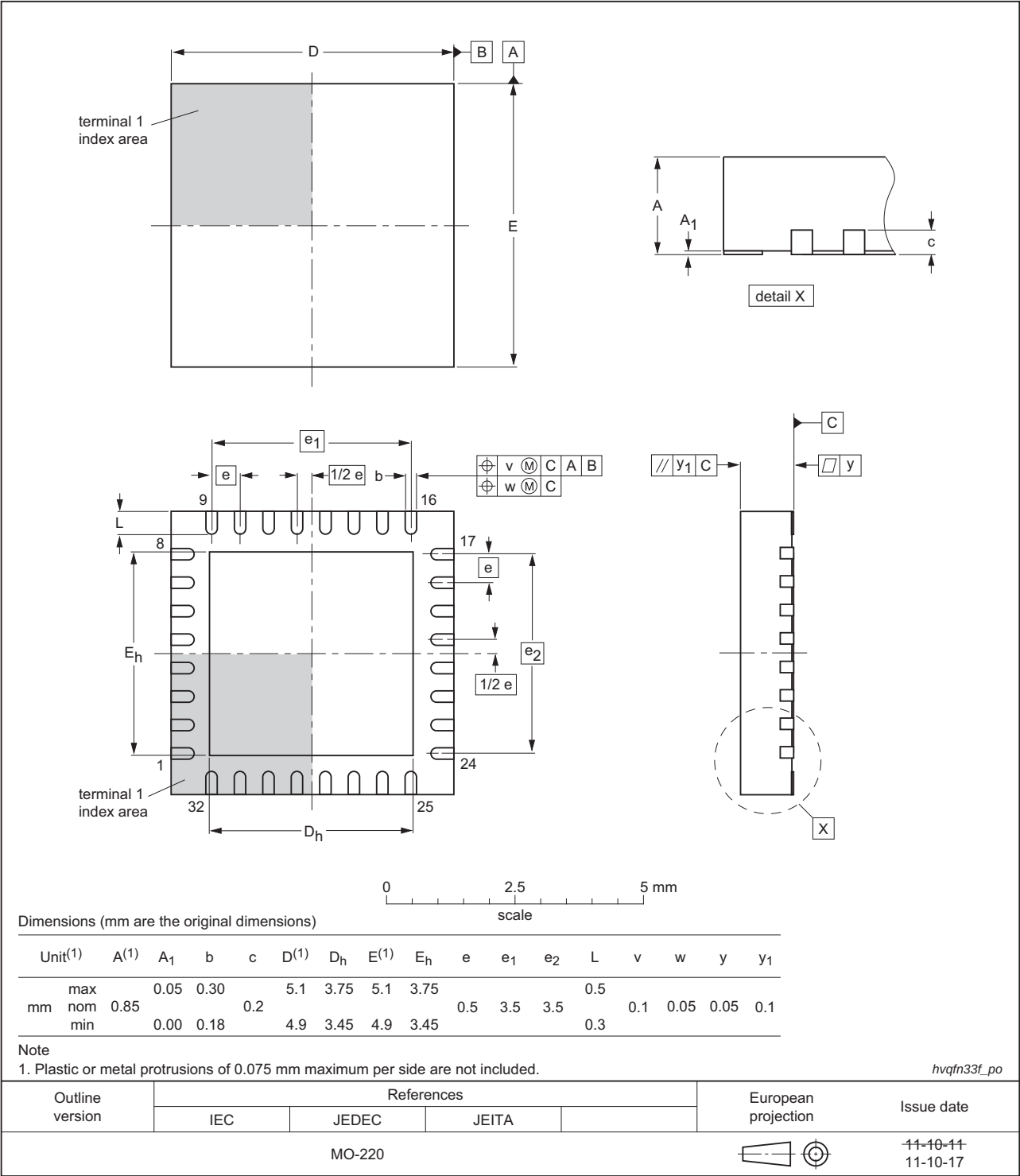
HVQFN33: plastic thermal enhanced very thin quad flat package; no leads; 32 terminals; body 5 x 5 x 0.85 mm
