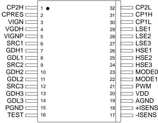
Figure 3. 33395 Pin Connections
