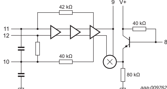
Fig 9. Second limiter and quadrature detector
