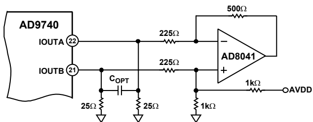
Figure 34. Single-Supply DC Differential Coupled Circuit
