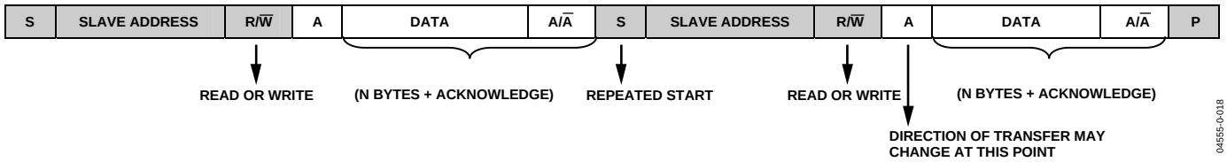
Figure 18. Combined Transmit/Read
