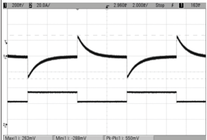
Step Load Transient Response ( V_{in}=48V , V_{out}=nom , C_{load}=1\mu F \parallel 10\mu F , I_{out}=50\% to 75% to 50% of full load, T_a=+25^\circ C ) Ch1= V_{out} , Ch2= I_{out}
