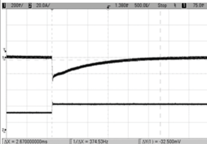
Step Load Transient Response ( V_{in}=48V , V_{out}=nom , C_{load}=1\mu F \parallel 10\mu F , I_{out}=50\% to 75% of full load, T_a=+25^\circ C ) Ch1= V_{out} , Ch2= I_{out}
