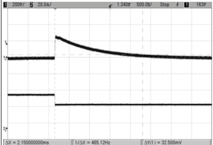
Step Load Transient Response ( V_{in}=48V , V_{out}=nom , C_{load}=1\mu F \parallel 10\mu F , I_{out}=75\% to 50% of full load, T_a=+25^\circ C ) Ch1= V_{out} , Ch2= I_{out}
