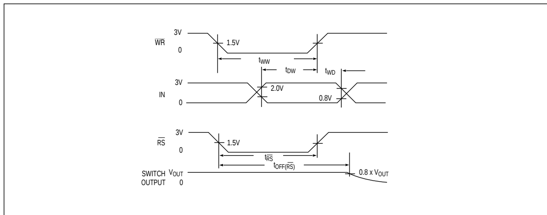
Figure 3. Latch Timing
