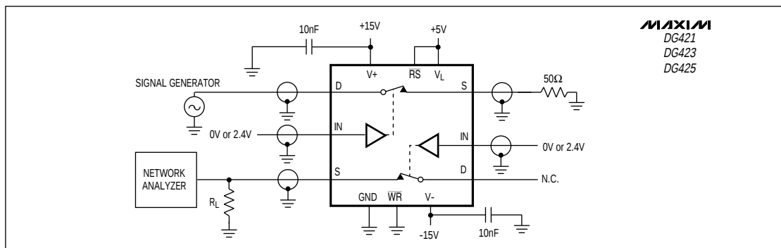
Figure 7. Crosstalk
