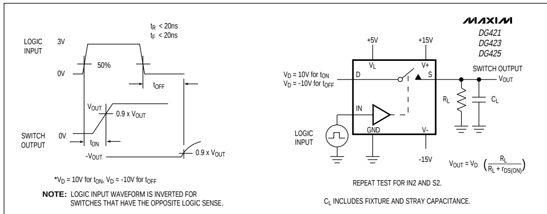
Figure 2. Switching Time
