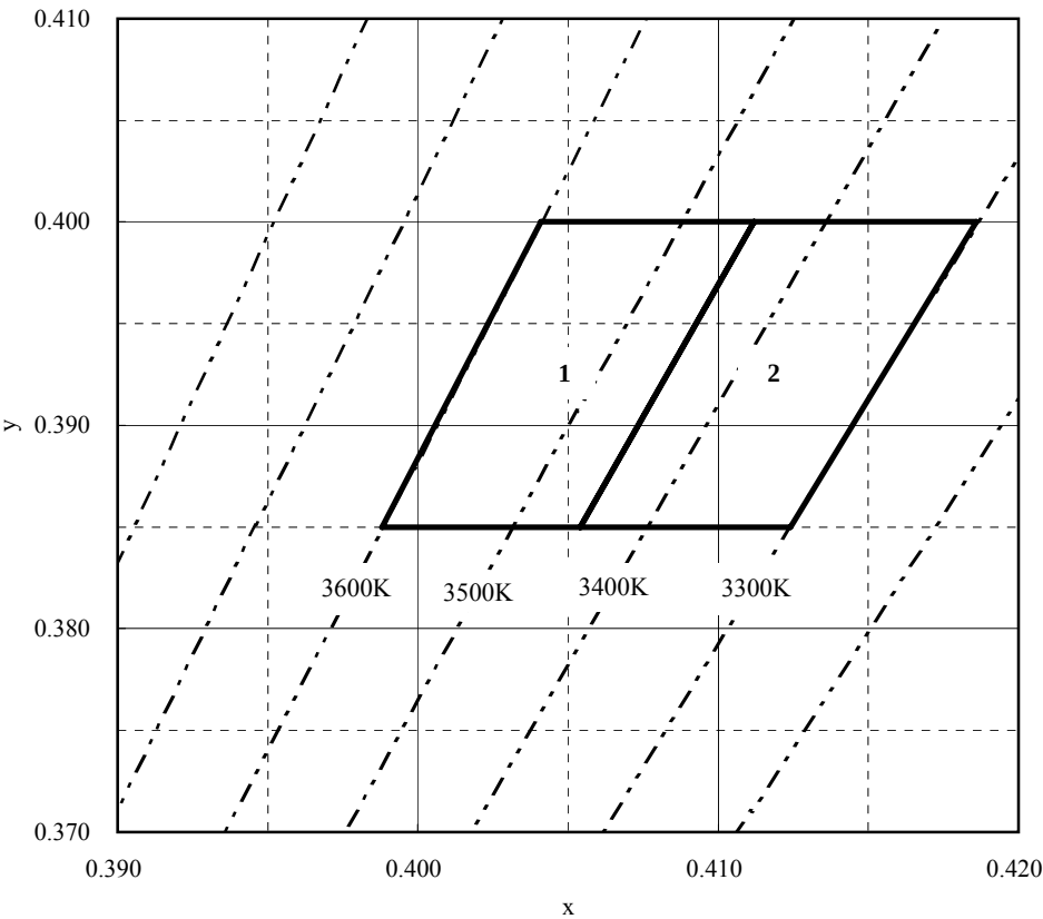
Chromaticity Diagram
