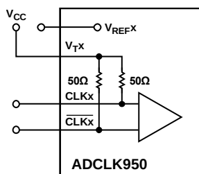
Figure 19. DC-Coupled CML Input Termination
