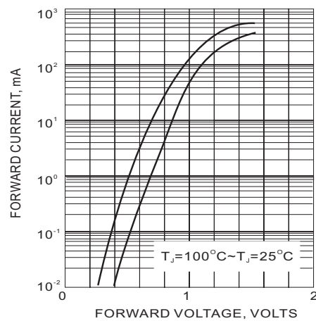
Fig.3 FORWARD CHARACTERISTICS
