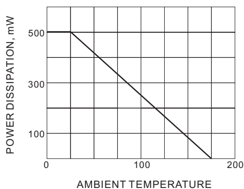
Fig.4 DERATING CURVE
