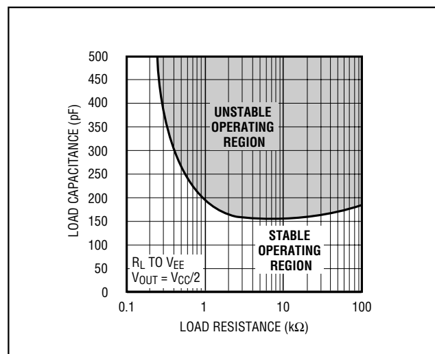
Figure 4. Capacitive-Load Stability
