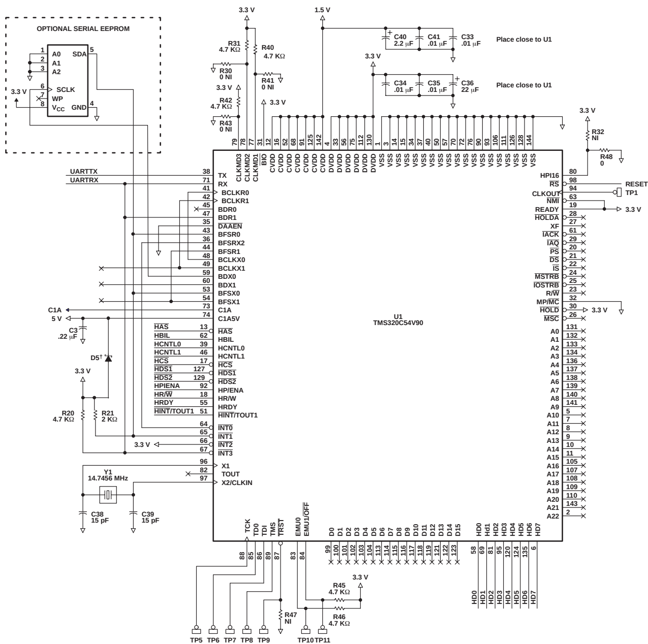
TMS320C54V90 SCHEMATIC
