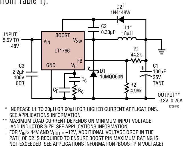
Figure 15. Positive-to-Negative Converter
