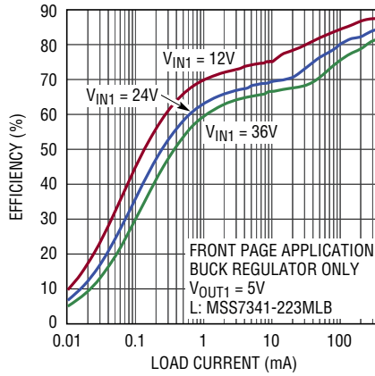
Efficiency, V_{OUT} = 5\text{V}
