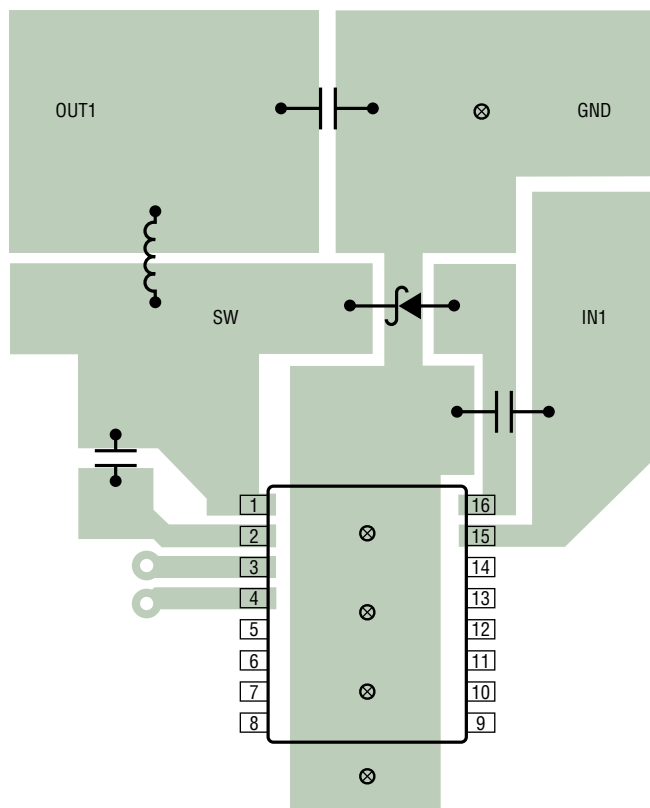
Figure 12. Good PCB Layout Ensures Proper, Low EMI Operation (MSOP)
