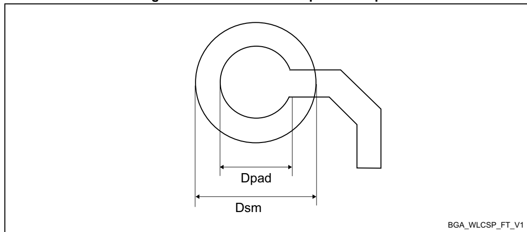
Figure 73. WLCSP156 - footprint example
