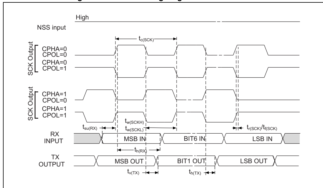
Figure 53. USART timing diagram in Master mode
