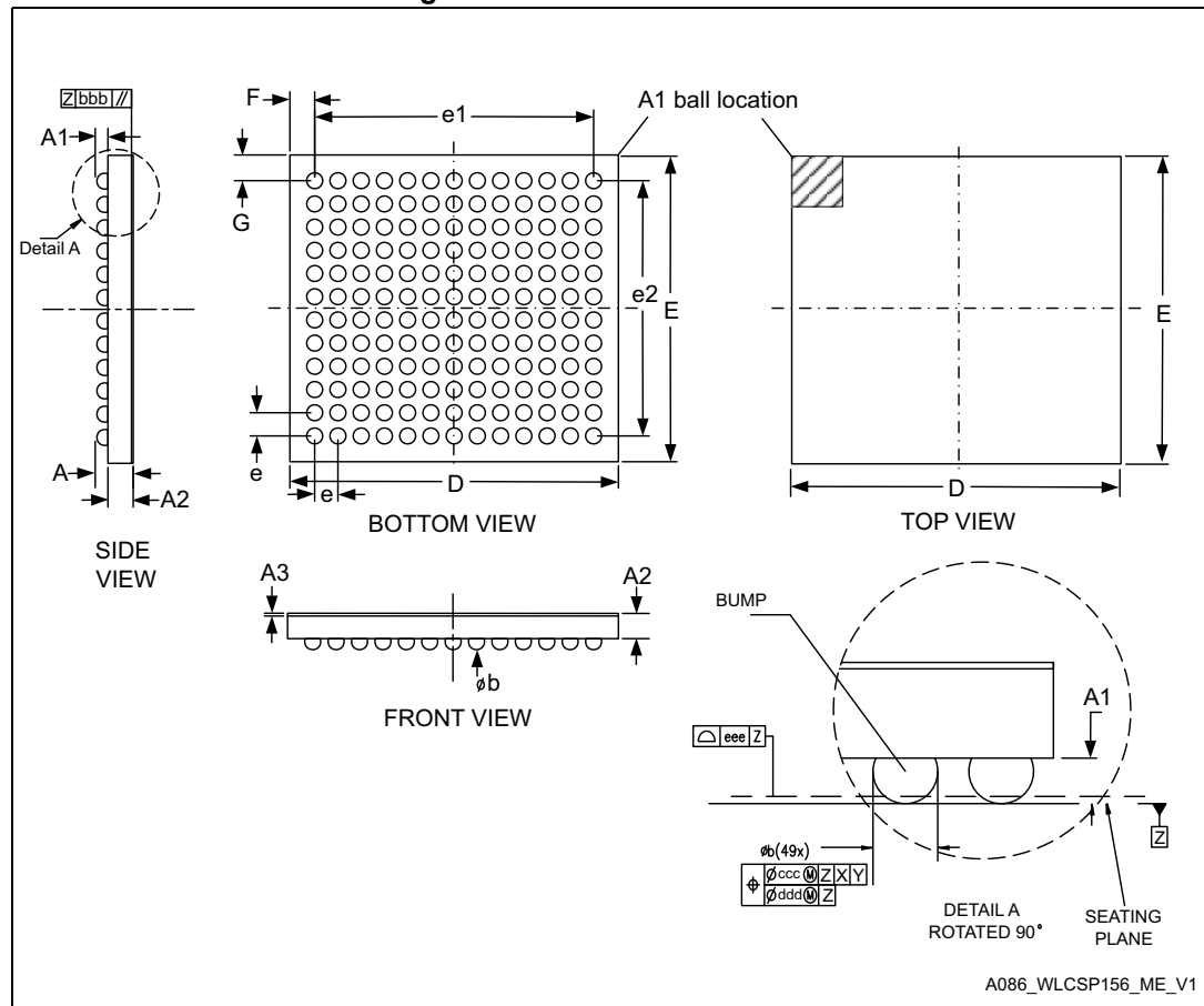
Figure 72. WLCSP156 - Outline
