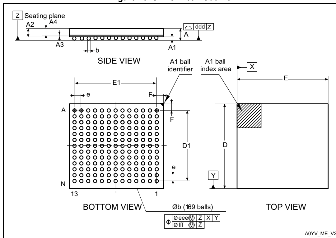
Figure 75. UFBGA169 - Outline
