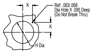
Recommended Panel Cut-out For Shell Sizes 20 Thru 24
