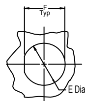
Recommended Panel Cut-out For Shell Sizes 08 Thru 18
