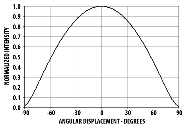
Figure 11. Radiation Pattern
