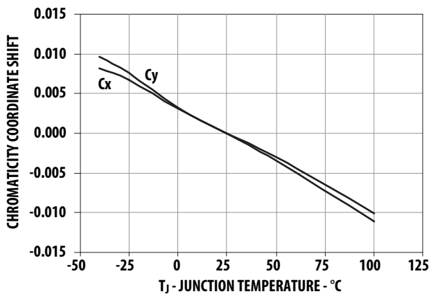
Figure 10. Chromaticity Shift Vs. Temperature
