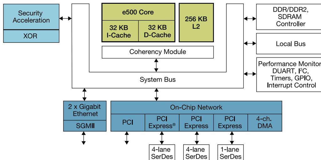
MPC8544E Block Diagram
