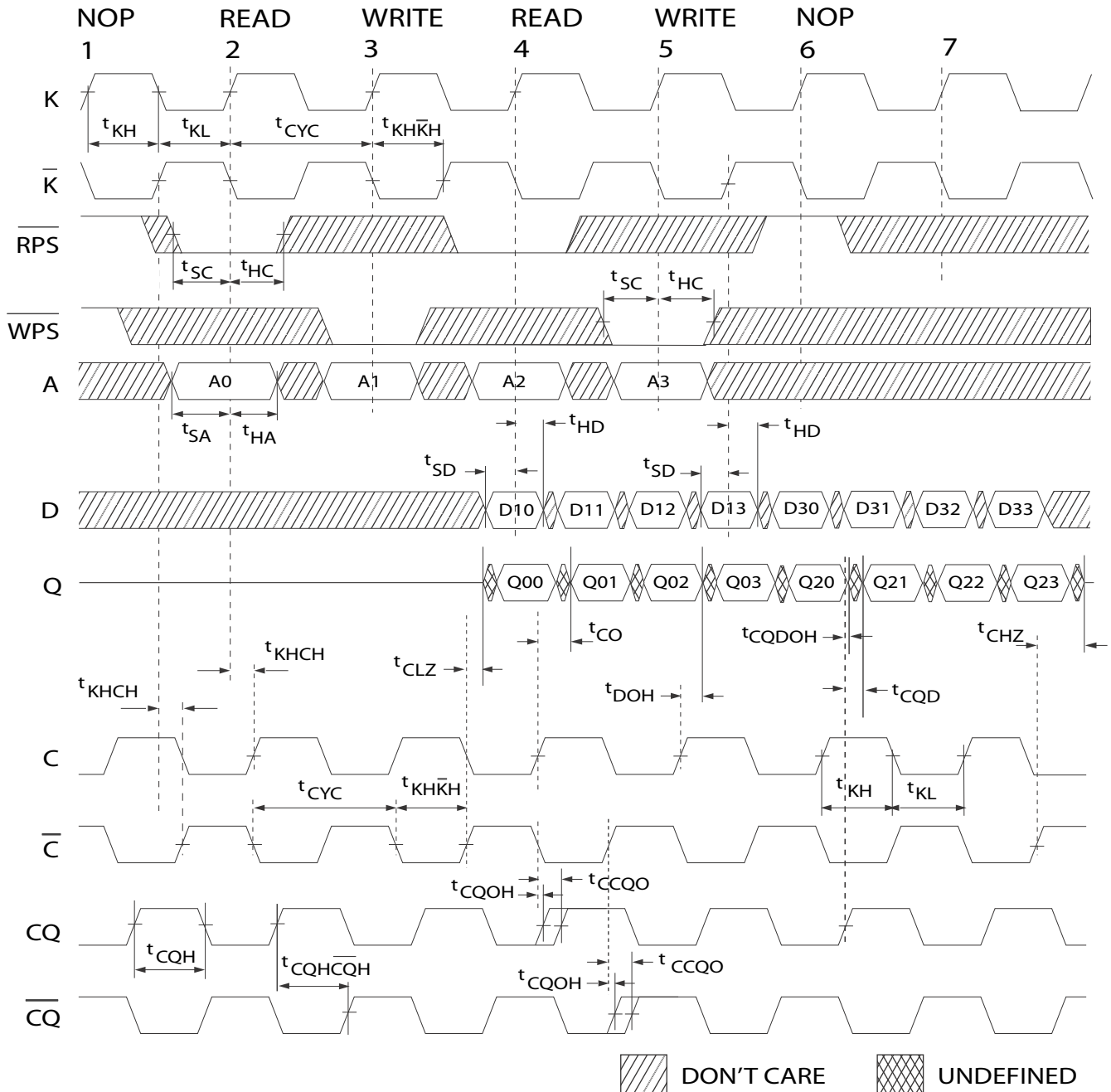
Figure 6. Read/Write/Deselect Sequence [37, 38, 39]
