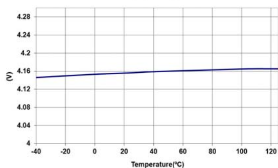
Vcc_UVLO_Start
