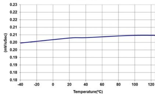
Ramp(SS_start)
