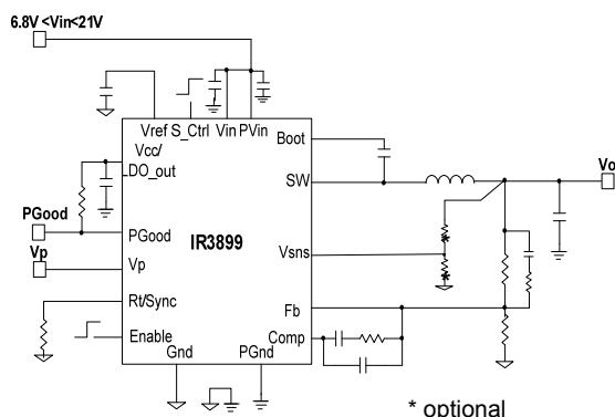
Figure 1: IR3899 Basic Application Circuit
