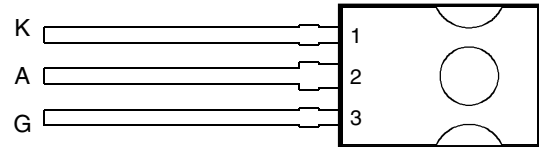
L PACKAGE (TOP VIEW)
