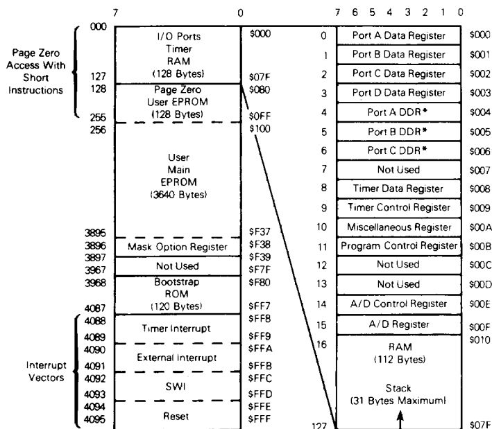
Figure 4. Memory Map
