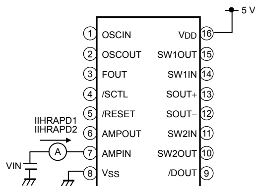
(18) Amplifier input sensitivity
