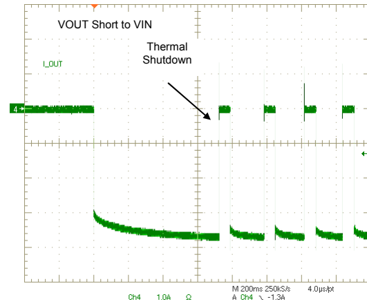
Current Limit Test (VIN=1.8V)
