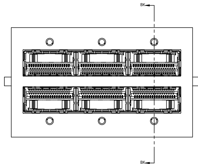
PART NUMBER SHOWN U90-G351-107A (WITH SINGLE BARREL ROUND LIGHT PIPE)
