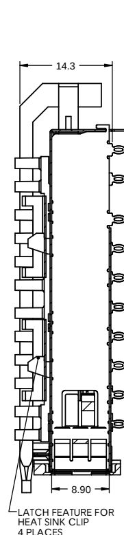
SECTION BB-BB SCALE 2.5 : 1
