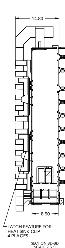
SECTION BD-BD SCALE 2.5:1
