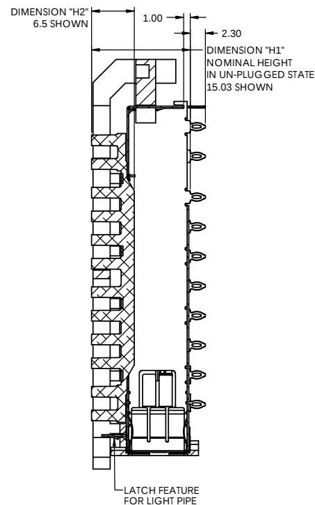
SECTION BE-BE SCALE 2.5:1
