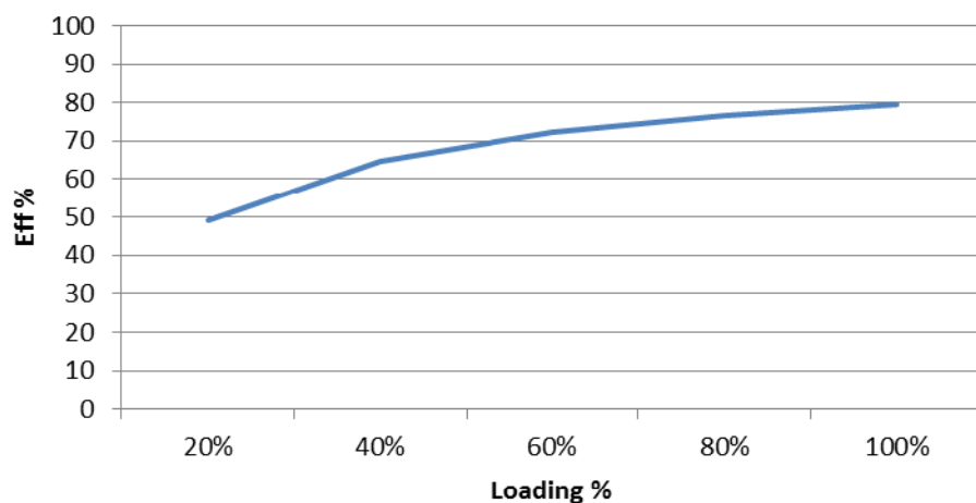
AM1DS-1212SZ Efficiency vs. Loading
