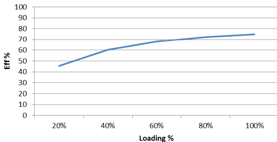
AM1DS-1505SZ Efficiency vs. Loading
