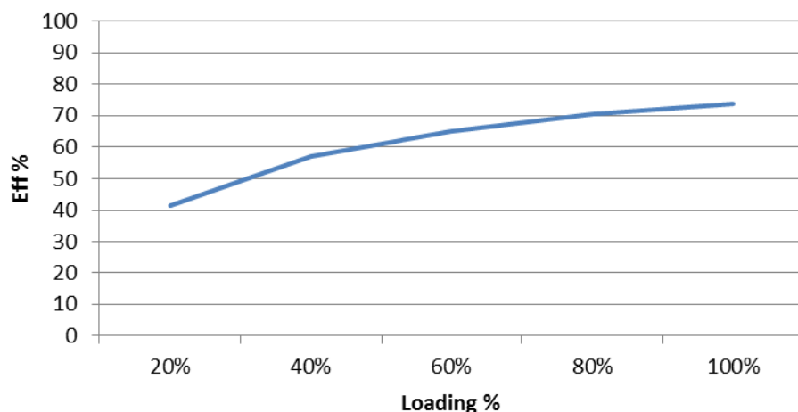
AM1DS-2412SZ Efficiency vs. Loading
