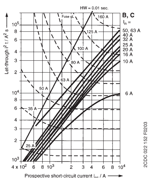
Miniature circuit-breakers S 200 M B/C
