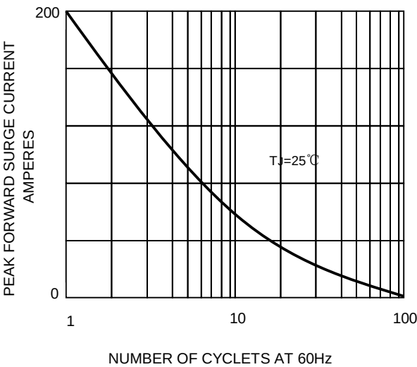
FIG.2-MAXIMUM FORWARD SURNGE CURRENT
