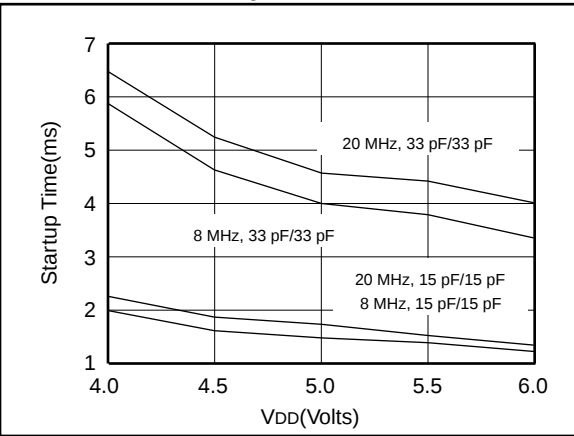
FIGURE 24-23: TYPICAL XTAL STARTUP TIME vs. VDD (HS MODE, 25°C)
