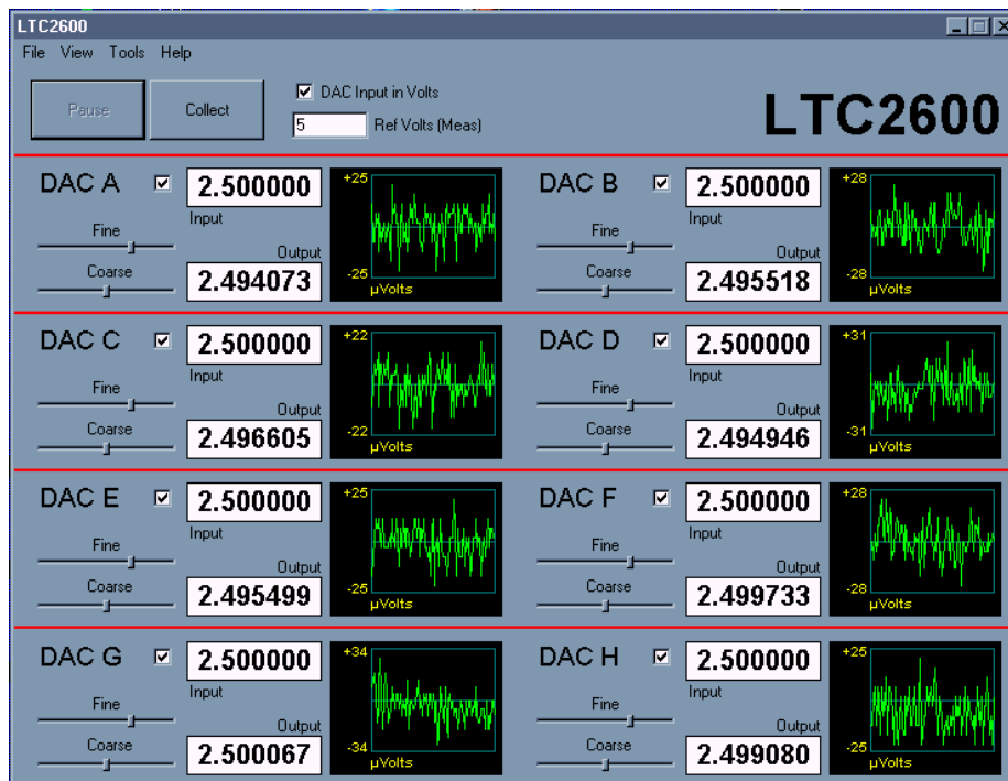
Figure 2. Evaluation Software
