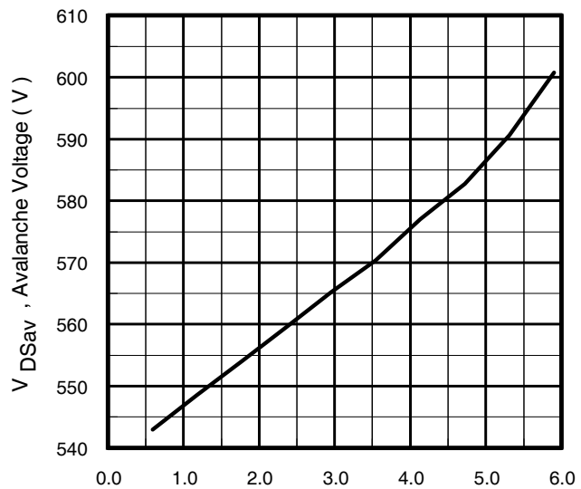
Fig 12d. Typical Avalanche Source Voltage Vs. Avalanche Current
