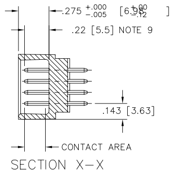
SECTION X-X
