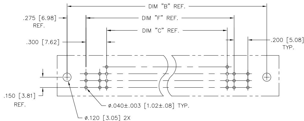
DETAIL P (INSTALLED IN PCB, NOTE 8)
